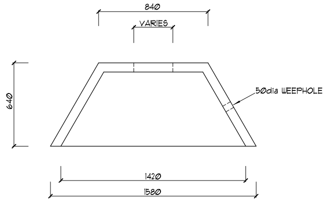
PLAN SCALE 1:25
